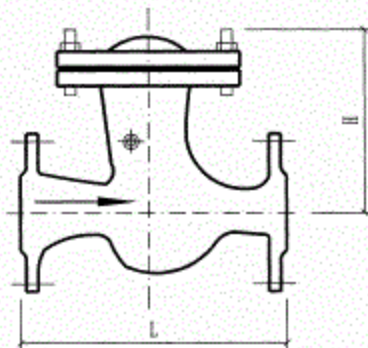
旋启式止回阀
