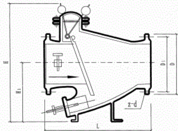
H44X-10 型缓闭止回阀
