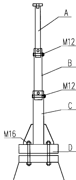
S3000 ,LCT针安装图
