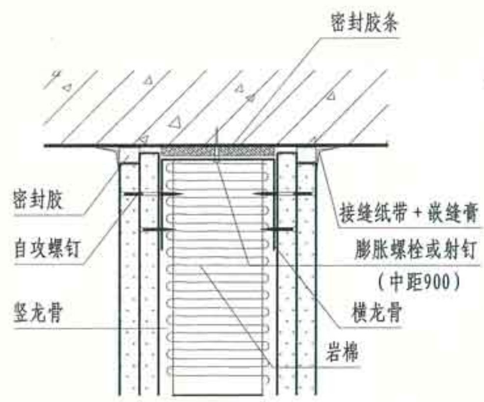
① 双层板、有隔音、带密封胶条
