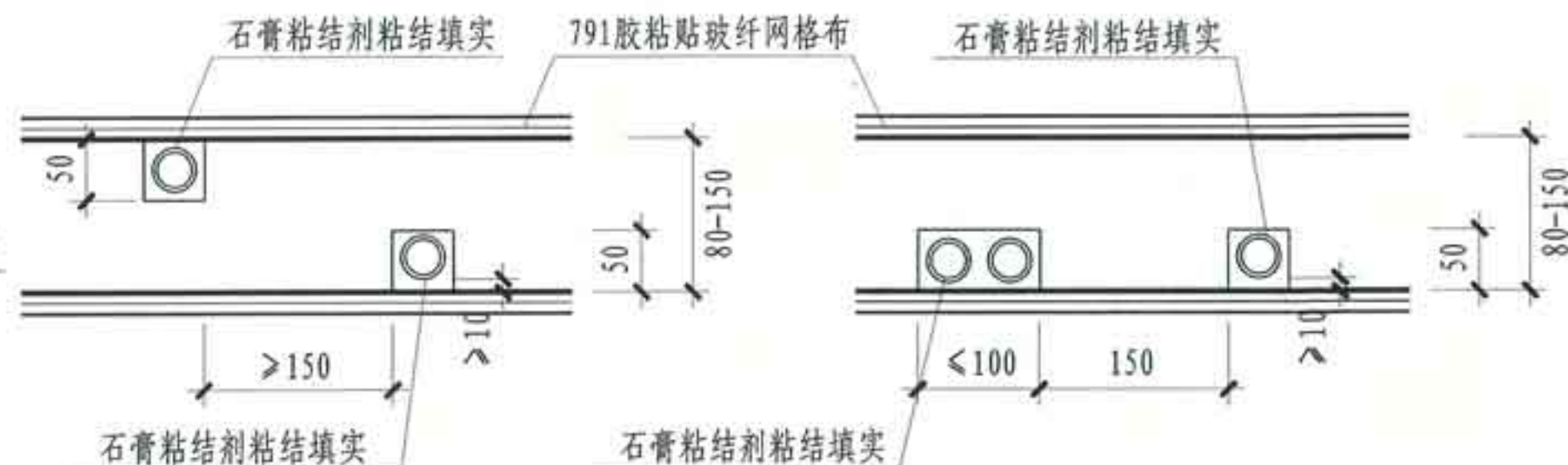
③ 竖向穿墙管槽
