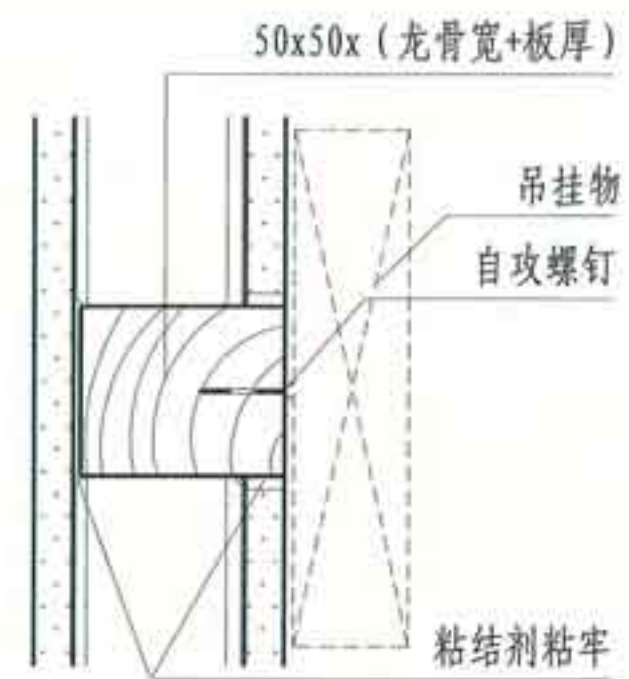
③ 粘结木块吊挂
