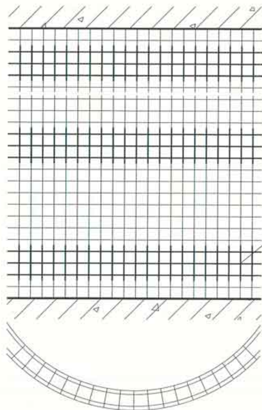
R \leq 500\text{cm} 弧面墙补强 (双面)
