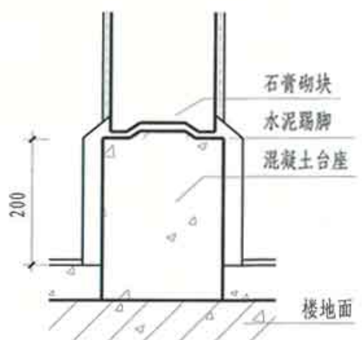
③ 砌块隔墙与楼、地面连接
