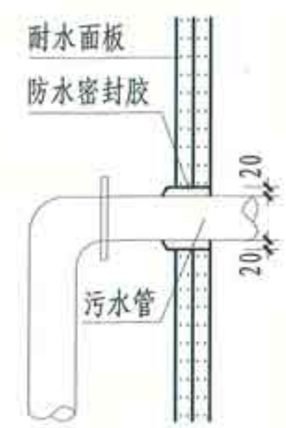
③ 坐便涉水管穿墙
