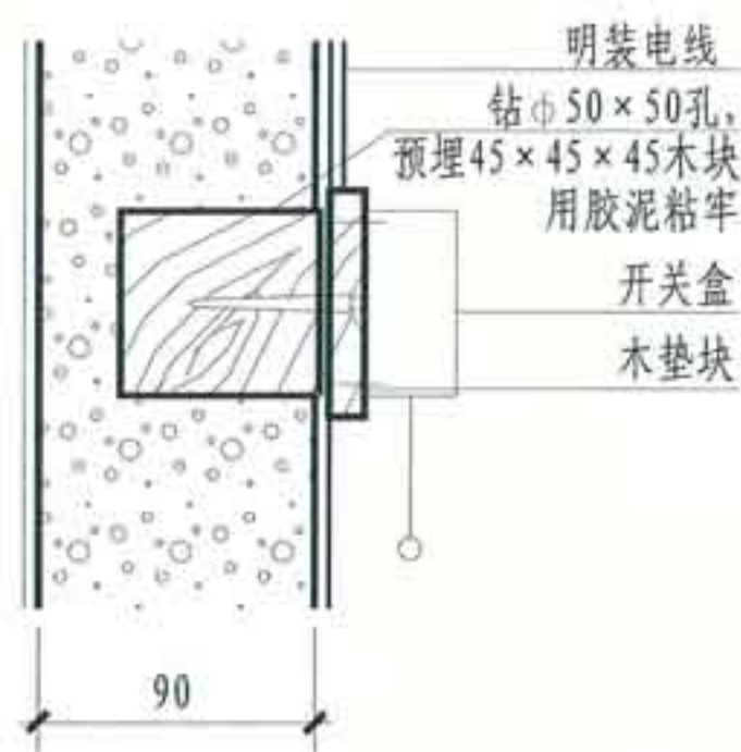
① 明线拉线开关
