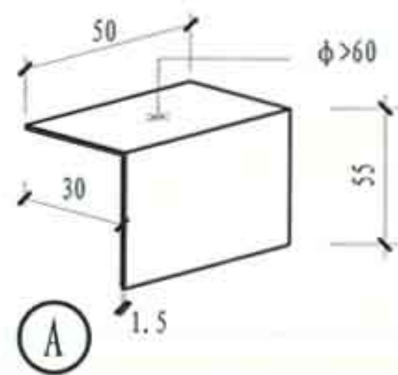
③ 砌块隔墙与楼、地面连接
