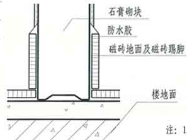
⑤ 砌块隔墙与楼、地面连接
