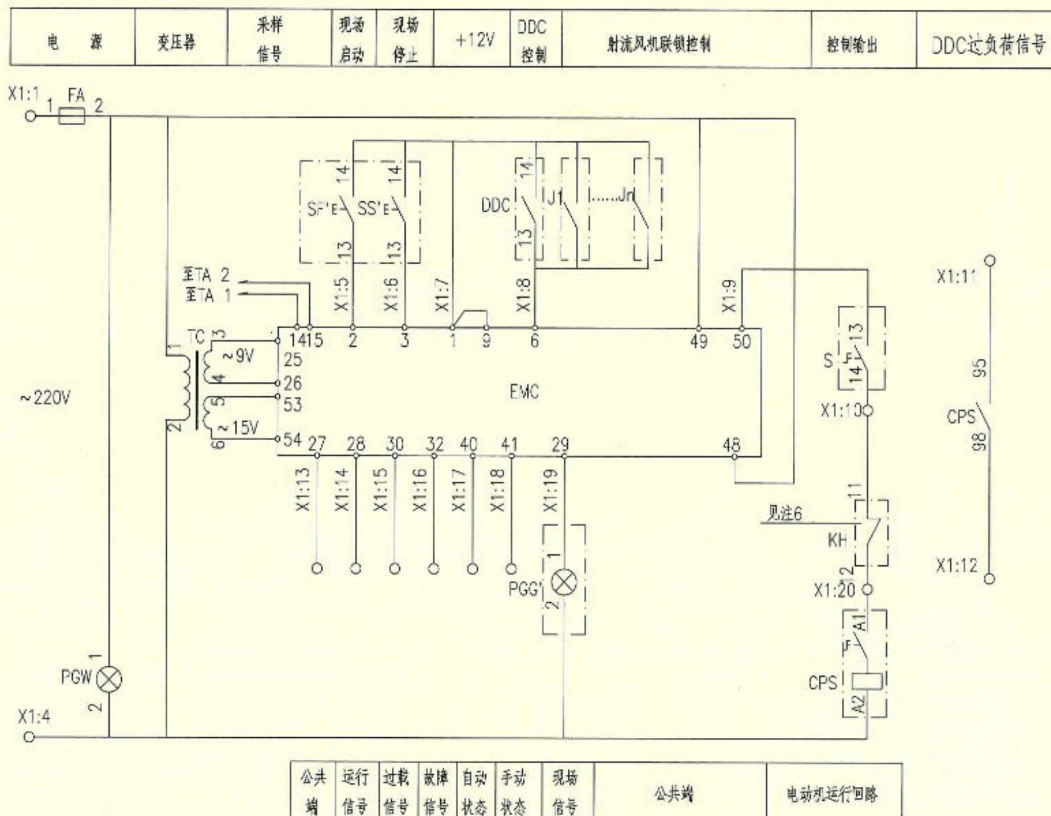
射流风机联锁排风机电路图 XKLF-4
