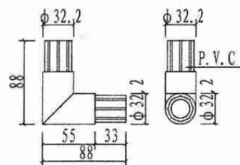
8 L型拉杆接头大样
