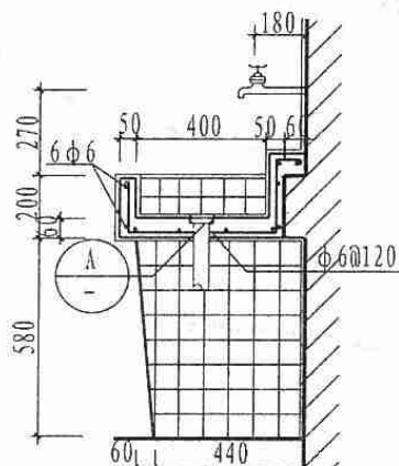
2-2
