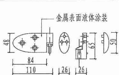
1 铰链大样
