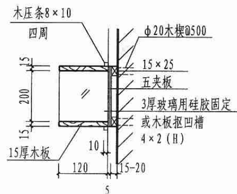
2-2
